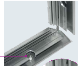
Detail of angle connector
