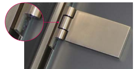
CODE 170.BB with safety fixing plate
